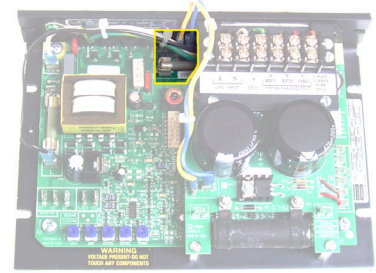
FIGURE 2. Location of motor fuse and quick connect tabs M+ and MF3.
